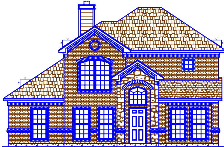
B FRONT ELEVATION SCALE: 1/4" = 1'-0"
