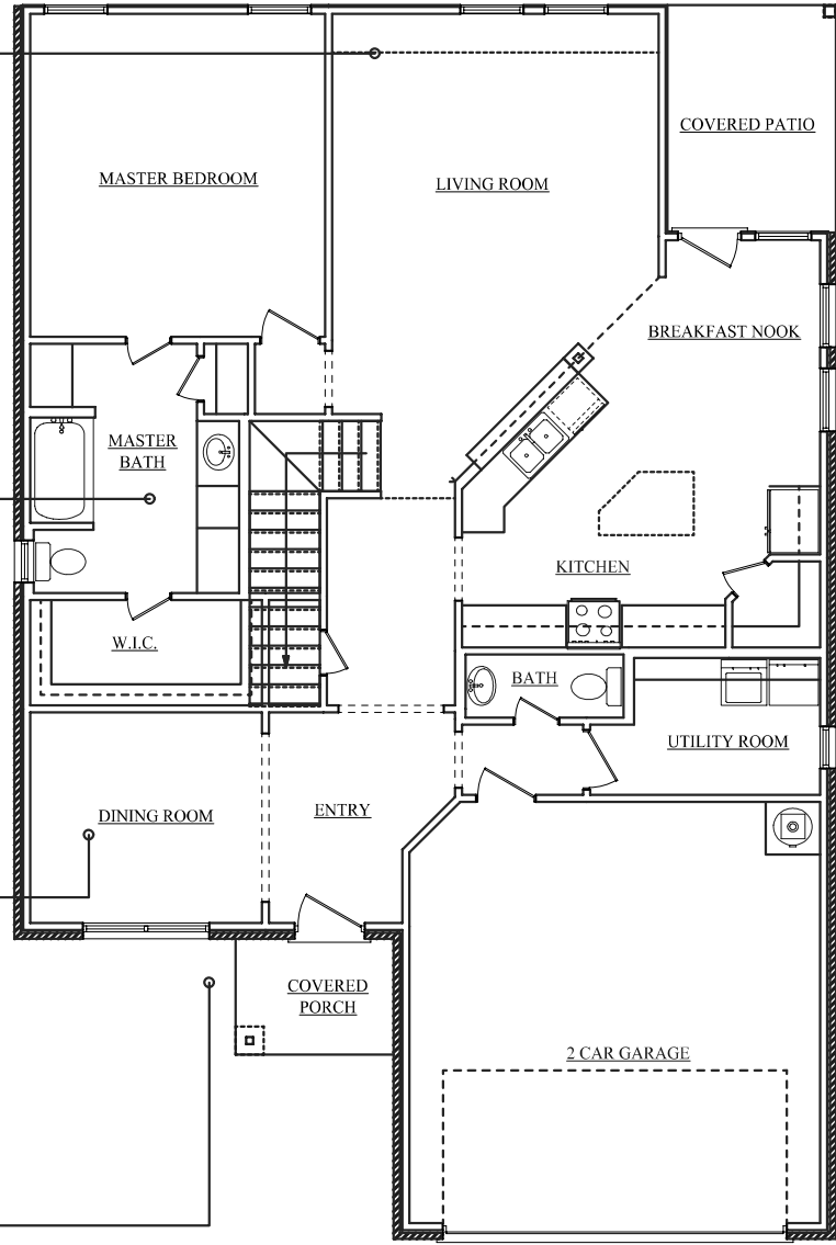
PLAN NAME: PRESTON PLAN ID: JH1-4411 2300 SQFT. A/C
